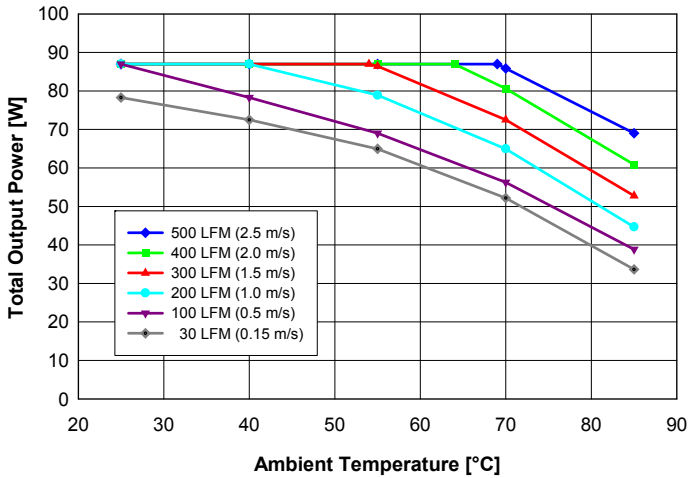
Fig. 8: Available output power for balanced load current ( I_{out1} = I_{out2} ) vs. ambient air temperature and airflow rates for converter mounted vertically with V_{in} = 48\text{ V} , air flowing from pin 3 to pin 1 and maximum FET temperature \leq 120^{\circ}\text{C} .
