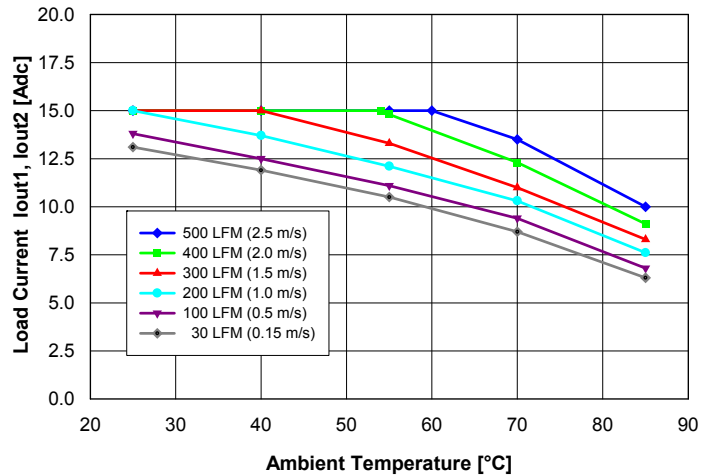
Fig. 11: Available balanced load current ( I_{out1} = I_{out2} ) vs. ambient temperature and airflow rates for converter mounted horizontally with V_{in} = 48\text{ V} , air flowing from pin 3 to pin 4 and maximum FET temperature \leq 120^{\circ}\text{C} .
