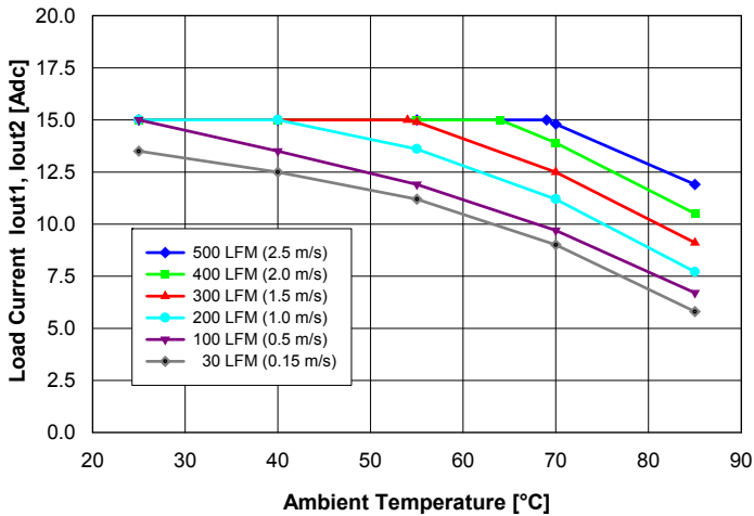
Fig. 10: Available balanced load current ( I_{out1} = I_{out2} ) vs. ambient air temperature and airflow rates for converter mounted vertically with V_{in} = 48\text{ V} , air flowing from pin 3 to pin 1 and maximum FET temperature \leq 120^{\circ}\text{C} .
