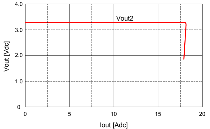
Fig. 27: Output voltage V_{out2} vs. load current I_{out2} showing current limit point and converter shutdown point. When V_{out2} is in current limit, V_{out1} is not affected until V_{out2} reaches the shut-down threshold equal to V_{out1} - 0.6 V. Input voltage has almost no effect on V_{out2} current limit characteristic.
