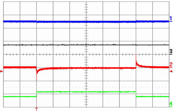
Fig. 23: Output voltage response to lout2 load current step-change of 3.75 A (50%-75%-50%) at lout1 = 7.5 A and Vin = 48 V. Ch1 = Vout1 (100 mV/div), Ch2 = Vout2 (100 mV/div), Ch3 = lout1 (10 A/div.), Ch4 = lout2 (10 A/div.). Current slew rate: 5 A/ \mu s, Co = 300 \mu F tantalum + 1 \mu F ceramic. Time scale: 0.5 ms/div.
