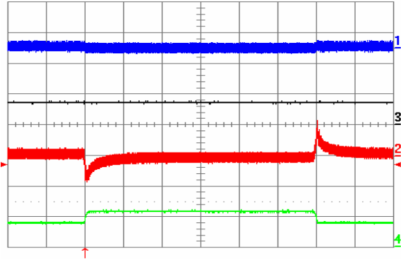
Fig. 21: Output voltage response to lout2 load current step-change of 3.75 A (50%-75%-50%) at lout1 = 7.5 A and Vin = 48 V. Ch1 = Vout1 (50 mV/div), Ch2 = Vout2 (50 mV/div), Ch3 = lout1 (10 A/div.), Ch4 = lout2 (10 A/div.). Current slew rate: 0.1 A/ \mu s, Co = 10 \mu F tantalum + 1 \mu F ceramic. Time scale: 0.5 ms/div.
