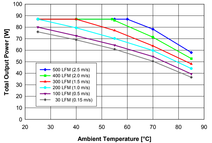
Fig. 9: Available output power for balanced load current ( I_{out1} = I_{out2} ) vs. ambient air temperature and airflow rates for converter mounted horizontally with V_{in} = 48\text{ V} , air flowing from pin 3 to pin 4 and maximum FET temperature \leq 120^{\circ}\text{C} .
