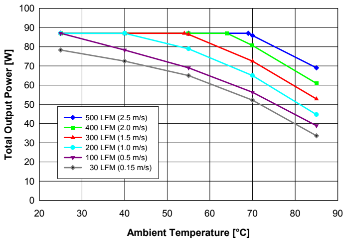
Fig. 1: Available output power vs. ambient air temperature and airflow rates for QD48T025033 converter mounted vertically with air flowing from pin 3 to pin 1, MOSFET temperature \leq 120^{\circ}\text{C} , V_{in} = 48\text{ V} and balanced load on both outputs ( I_{out1} = I_{out2} ).
