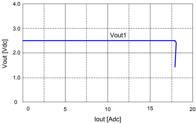
Fig. 26: Output voltage V_{out1} vs. load current I_{out1} showing current limit point and converter shutdown point. When V_{out1} is in current limit, V_{out2} is not affected until V_{out1} reaches the shut-down threshold of 60% of its nominal value. Input voltage has almost no effect on V_{out1} current limit characteristic.
