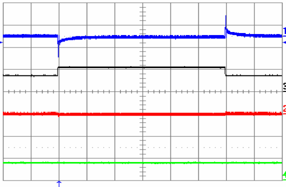
Fig. 22: Output voltage response to lout1 load current step-change of 3.75 A (50%-75%-50%) at lout2 = 7.5 A and Vin = 48 V. Ch1 = Vout1 (100 mV/div), Ch2 = Vout2 (100 mV/div), Ch3 = lout1 (10 A/div.), Ch4 = lout2 (10 A/div.). Current slew rate: 5 A/ \mu s, Co = 300 \mu F tantalum + 1 \mu F ceramic. Time scale: 0.5 ms/div.
