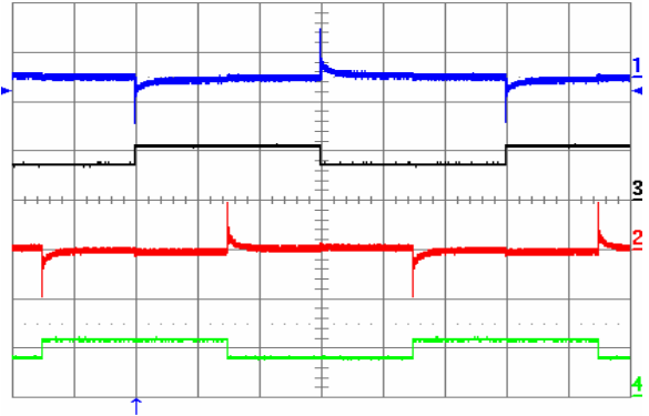
Fig. 25: Output voltage response to both I_{out1} and I_{out2} (out of phase) load current step-change of 3.75 A (50%-75%-50%) at V_{in} = 48 V. Ch1 = V_{out1} (100 mV/div), Ch2 = V_{out2} (100 mV/div), Ch3 = I_{out1} (10 A/div.), Ch4 = I_{out2} (10 A/div.). Current slew rate: 5 A/ \mu s, C_o = 300 \mu F tantalum + 1 \mu F ceramic. Time scale: 1 ms/div.
