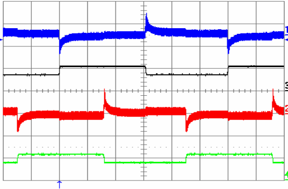
Fig. 24: Output voltage response to both I_{out1} and I_{out2} (out of phase) load current step-change of 3.75 A (50%-75%-50%) at V_{in} = 48 V. Ch1 = V_{out1} (50 mV/div), Ch2 = V_{out2} (50 mV/div), Ch3 = I_{out1} (10 A/div.), Ch4 = I_{out2} (10 A/div.). Current slew rate: 0.1 A/ \mu s, C_o = 10 \mu F tantalum + 1 \mu F ceramic. Time scale: 1 ms/div.
