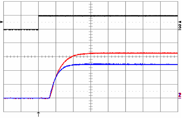
Fig. 19: Turn-on transient waveforms at full rated load current (resistive) and V in = 48 V, triggered via ON/OFF pin. Top trace: ON/OFF signal (5 V/div.). Bottom traces: V out1 (blue, 1 V/div.), V out2 (red, 1 V/div.). Time scale: 1 ms/div.
