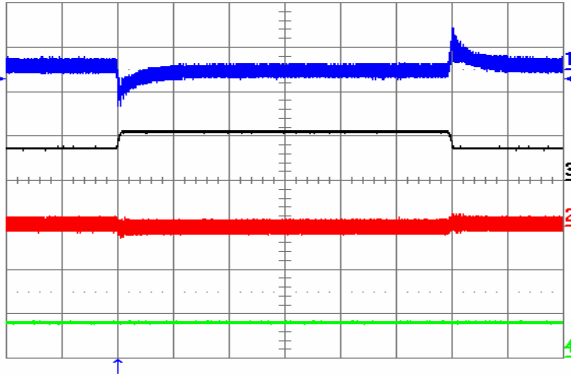
Fig. 20: Output voltage response to lout1 load current step-change of 3.75 A (50%-75%-50%) at lout2 = 7.5 A and Vin = 48 V. Ch1 = Vout1 (50 mV/div), Ch2 = Vout2 (50 mV/div), Ch3 = lout1 (10 A/div.), Ch4 = lout2 (10 A/div.). Current slew rate: 0.1 A/ \mu s, Co = 10 \mu F tantalum + 1 \mu F ceramic. Time scale: 0.5 ms/div.
