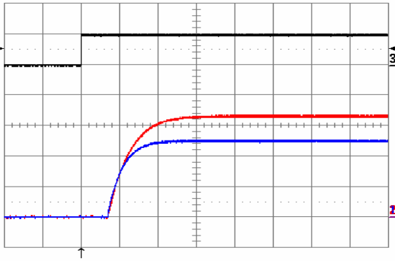
Fig. 18: Turn-on transient waveforms at no load current and V in = 48 V, triggered via ON/OFF pin. Top trace: ON/OFF signal (5 V/div.). Bottom traces: V out1 (blue, 1 V/div.), V out2 (red, 1 V/div.). Time scale: 1 ms/div.
