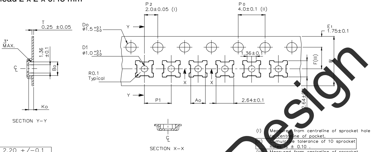
Figure 24. Tape and Reel Specifications 10-lead 2 x 2 x 0.45 mm
