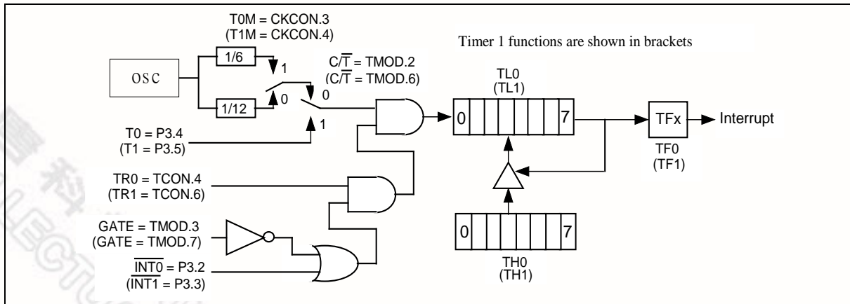
Figure 9-2 Timer/Counter Mode 2
