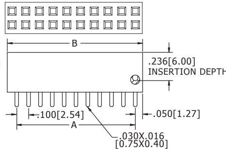
DUAL READOUT, STRAIGHT TAIL SHOWN
