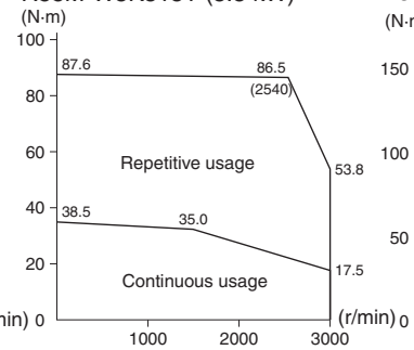
R88M-W5K515T (5.5 kW)
